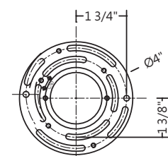
Mounting Ring Dimensions
