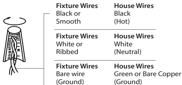
FIG.4 Driver Wiring
