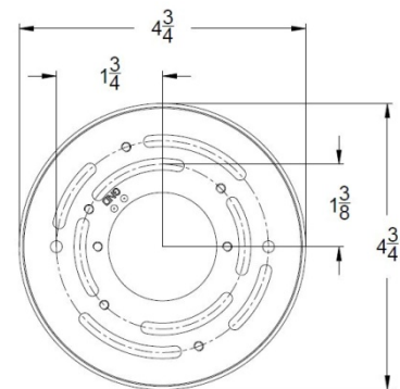
Back Ring Dimensions
