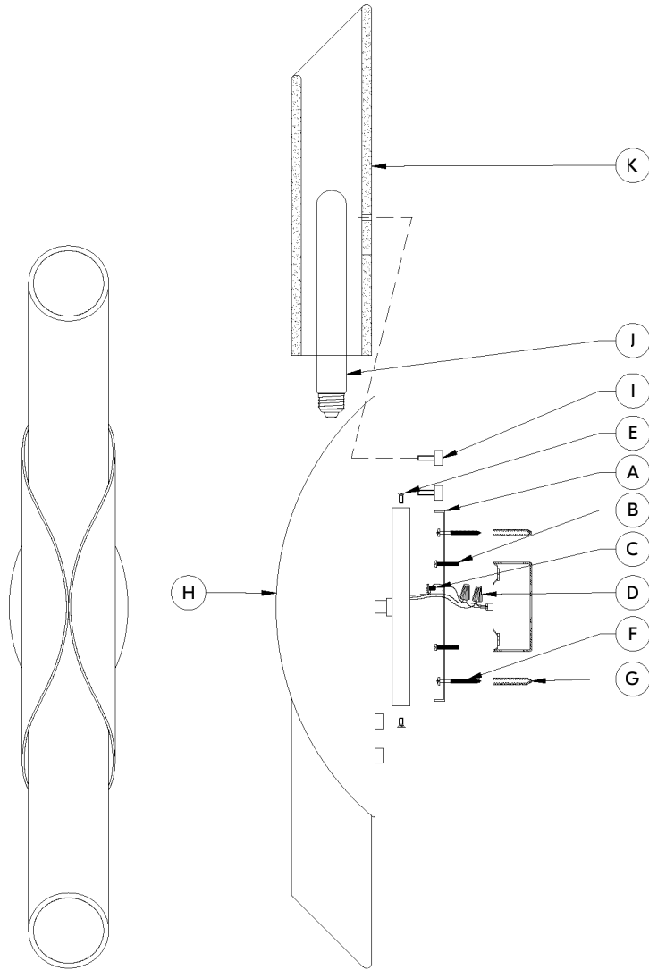
FRONT VIEW
