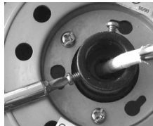
loosen set screws on coupler
