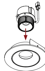
Attach LED module/driver
