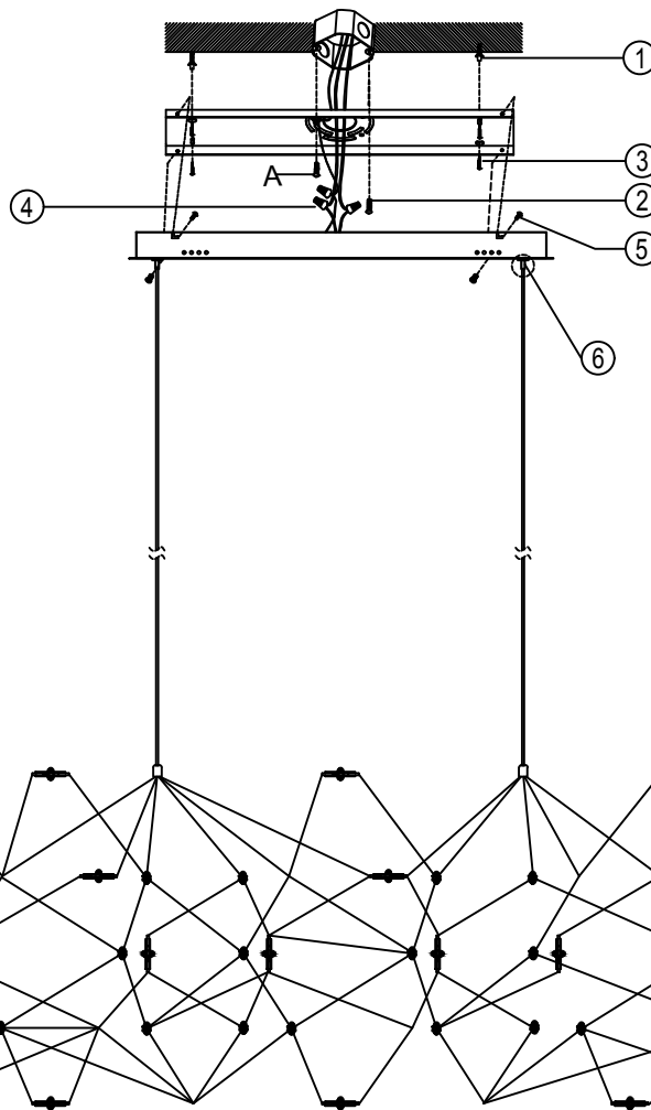
Wire connection
