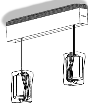
INSTALLATION WITHOUT ACCESSORY JUNCTION BOX
